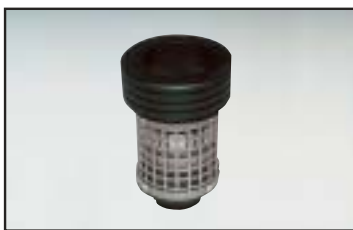
Protective valve. For safe lifts using fixed hooks/tools. Fitted between the lift tube and the vacuum box. Immediately eliminates the depression inside the lift tube if the load is released inadvertently.
